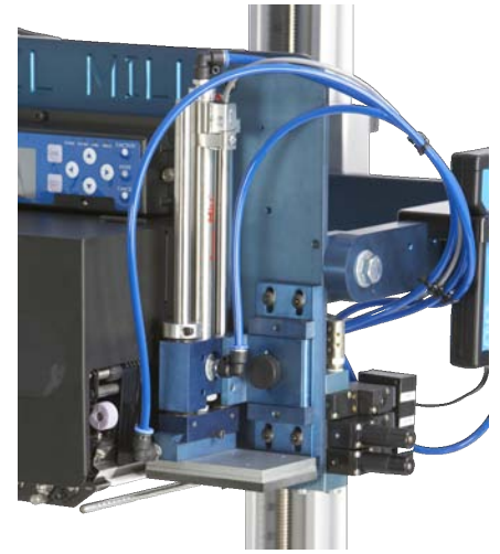
600 Printer Applicator with Tamp Module
